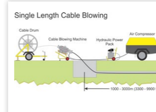
CABLE BLOWING
